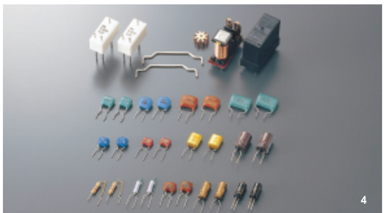
(1) Anti-Resonance Aluminum-Extruded Heat Sinks with High Efficient Cooling System (2) Extra-Large (4.7kg), Low-Impedance Transformer (3) Extra-Large Custom-Made Block Electrolytic Capacitors (4) FE Mica Capacitors, Polypropylene Film Capacitors, Polyethylene Telephthalate Capacitors, High Quality Resistors and Twin Direct Signal Path Speaker Relays with Gold-Plated Crossover Connection and Shielding
