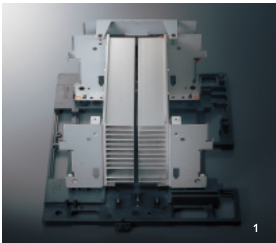
(1) Anti-Resonance Aluminum-Extruded Heat Sinks with High Efficient Cooling System (2) Extra-Large (4.7kg), Low-Impedance Transformer (3) Extra-Large Custom-Made Block Electrolytic Capacitors (4) FE Mica Capacitors, Polypropylene Film Capacitors, Polyethylene Telephthalate Capacitors, High Quality Resistors and Twin Direct Signal Path Speaker Relays with Gold-Plated Crossover Connection and Shielding
