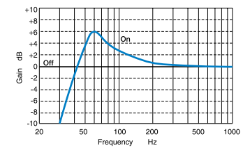
Bass Extension Characteristics
